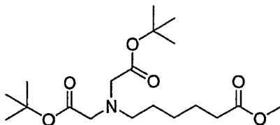
6-(Bis-tert-butoxycarbonylmethyl-amino)-hexanoic acid methyl ester
